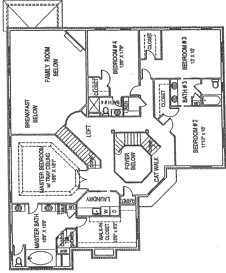
SECOND FLOOR 2308 SQ. FT.
